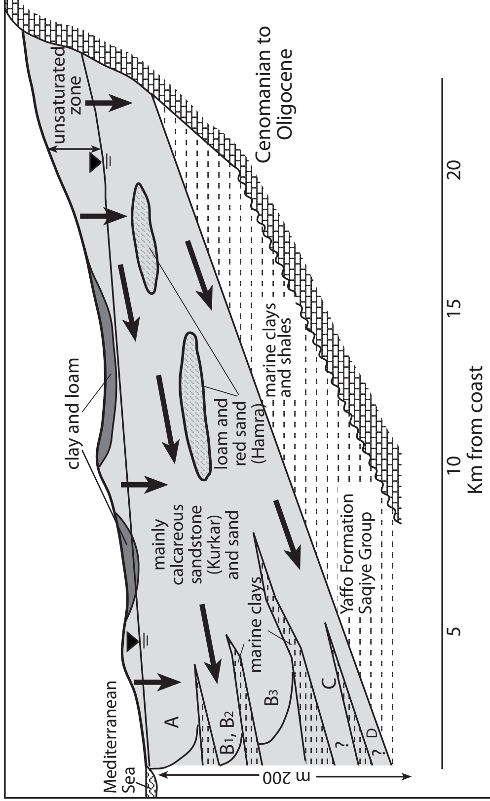
Schematic hydrogeological cross-section of the coastal aquifer of Israel. Arrows denote main directions of water flow.
